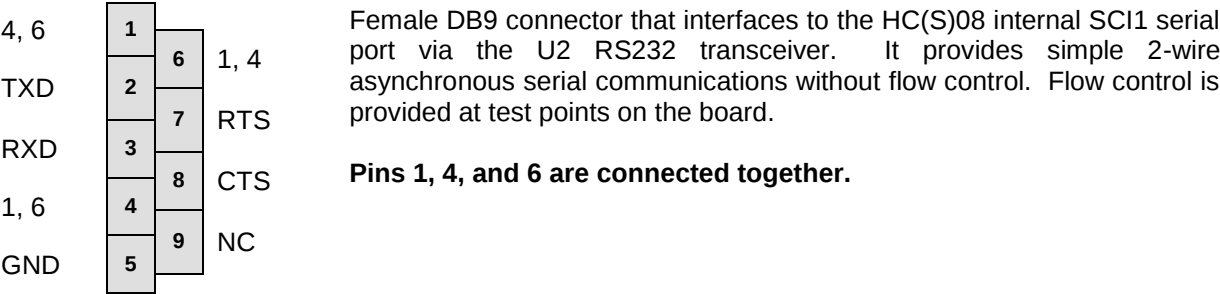
Figure 7: COM Connector
